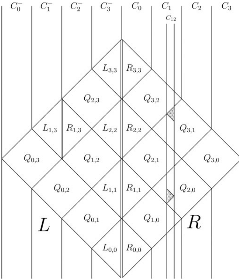
Fig. 1. The case M = 4 . The square Q split into two triangles L and R with level 1 squares, triangles, and columns. Also shown is level 2 column C_{12} with a \Delta -pair.
