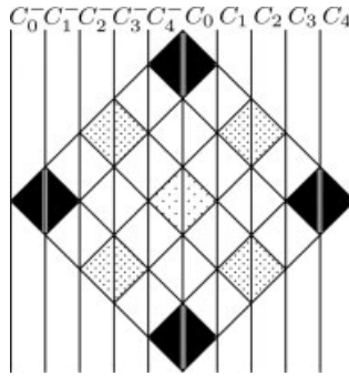
Fig. 2. The square Q for the (1, 0, \rho, 0, 1) Cantor set; the shades indicate the probabilities with which the Q_{i,j} do occur.
